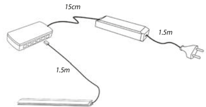
Image shows how this product is wired to a driver
