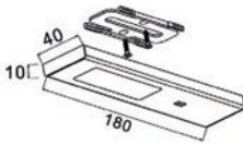
Under cabinet mounting (bracket provided with each fitting)
