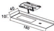
Under cabinet mounting (bracket provided with each fitting)
