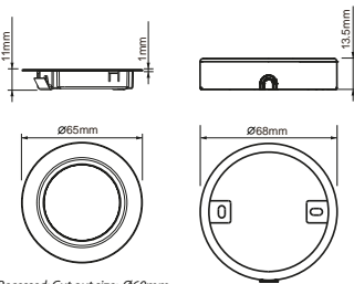
Recessed: Cut out size: Ø60mm
