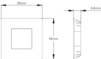
Cut out size: Ø44mm
