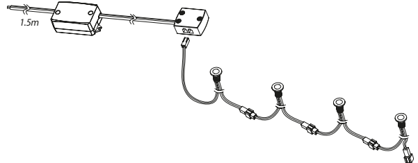
Image shows how this product is wired to a driver
