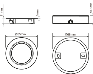
Recessed: Cut out size: Ø60mm
